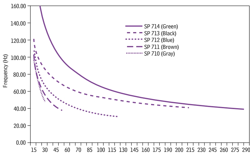
Fn vs. Stress Machine Pads
