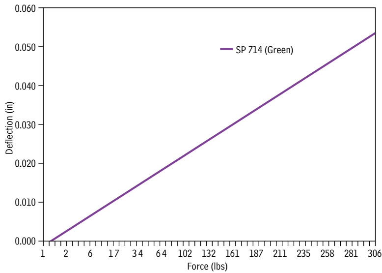
Load vs. Deflection Standard Machine Pad
