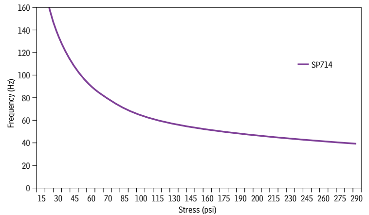
Fn vs. Stress MHD Machine Mount
